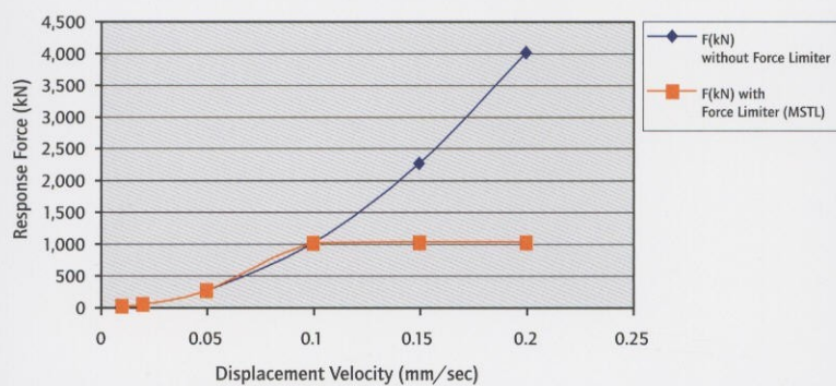
Force vs. velocity graph of a 1,000 kN shock transmitter with and without force limiter (MSTL) that deploy their design force at 0.1 mm/sec
