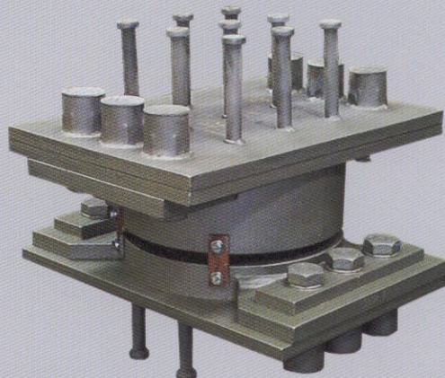
MSM® bearings for the Maglev Train in Shanghai
