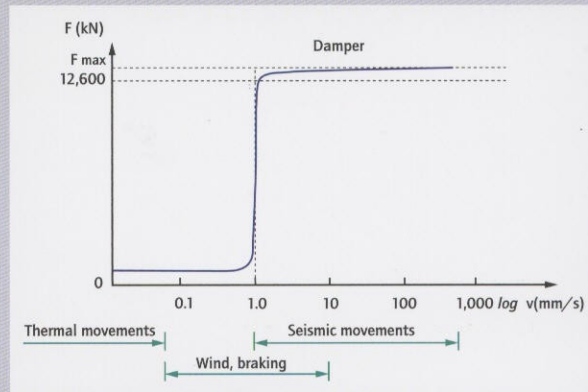
Actual characteristic force vs. velocity curve of a 12,600 kN hydraulic damper equipped with shock-transmission function
